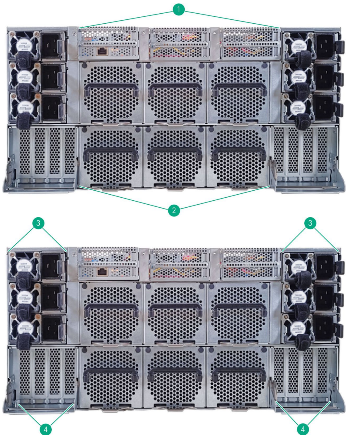
HPE Cray XD670 Server Rear View
