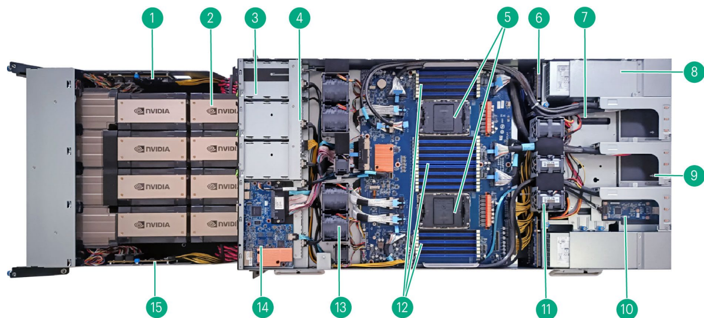
HPE Cray XD670 Server Top View
